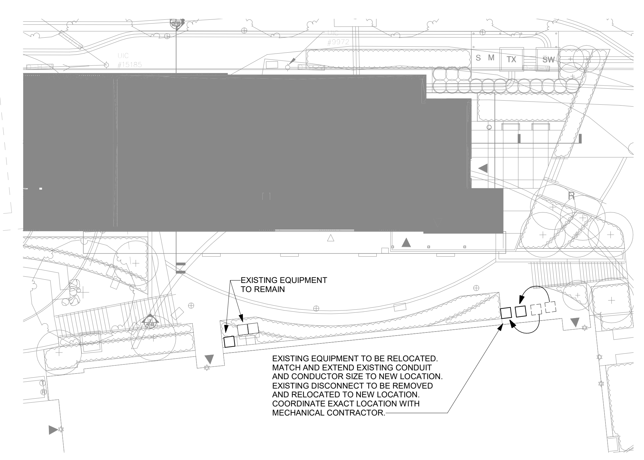
2 PELTZ GYM - PART PLAN ELECTRICAL 1" = 20'-0"
